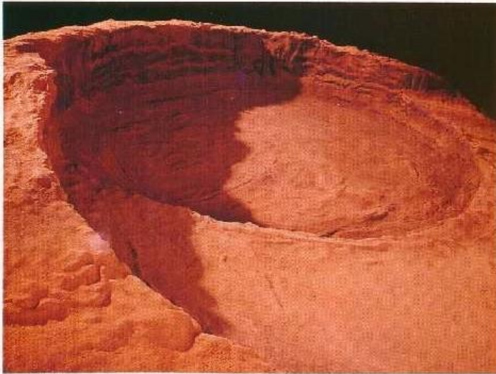
Mars Round Crater
